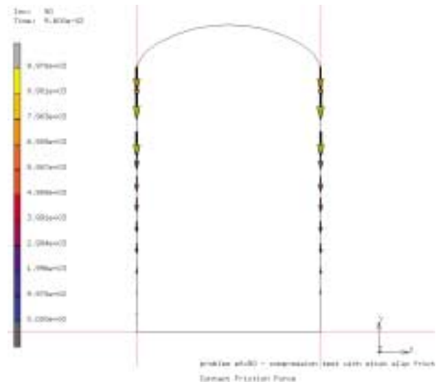
CONTACT FRICTION FORCE
