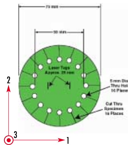
BIAXIAL SPECIMEN
