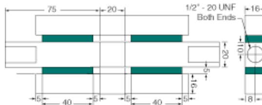
QUAD LAP SHEAR TEST
