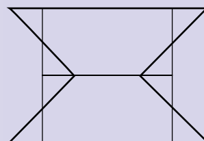
2-D HOURGLASSING MODE
