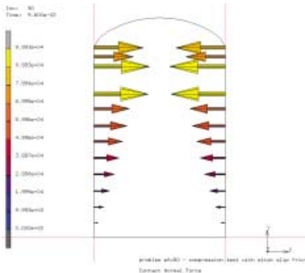
CONTACT NORMAL FORCE
