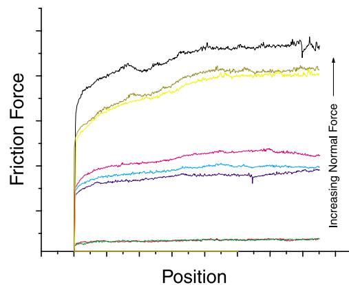
FRICTION DATA
