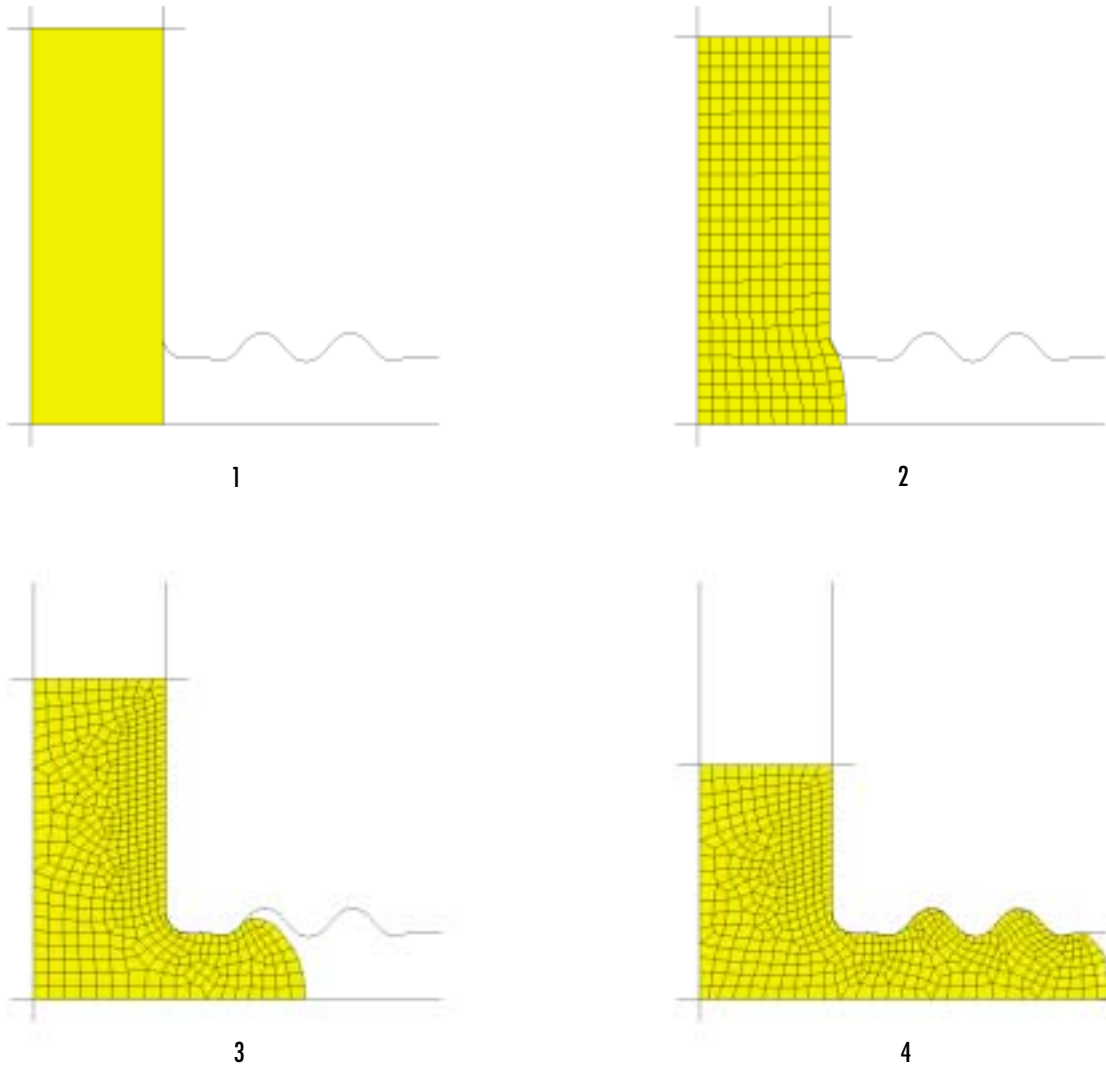
AUTOMATIC REMESHING AND REZONING OF A RUBBER SEAL
