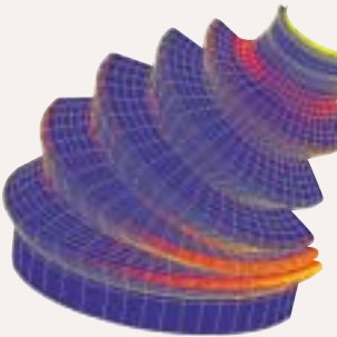
AXIAL COMPRESSION (INCREMENT 13)
