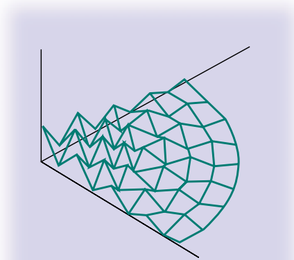
3-D HOURGLASSING: "EGGCRATE" MODE
